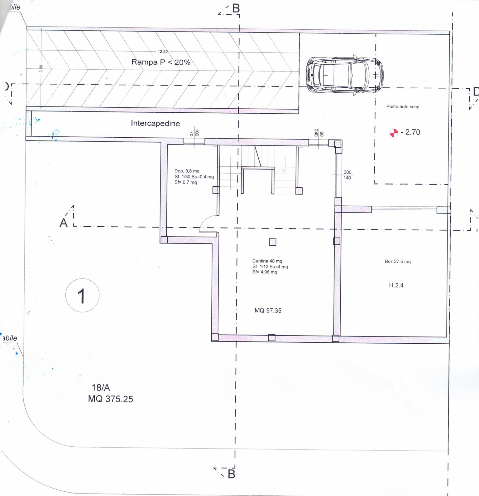
Planimetria Piano Inter.
