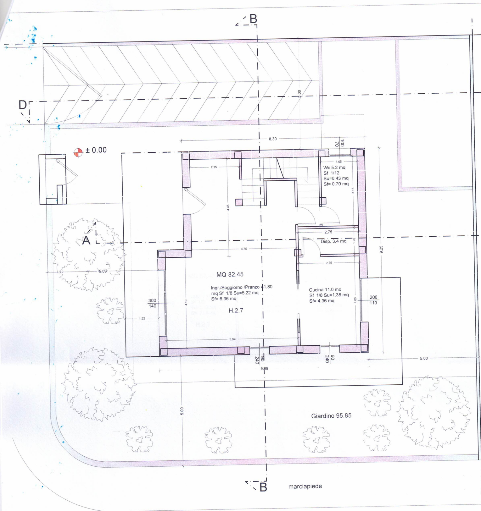
Planimetria Piano Terra
